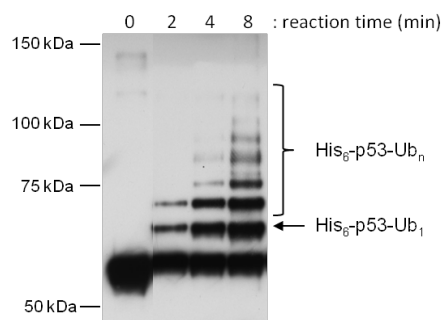
Figure 1: Ubiquitination of p53 by the MDM2 E3 ligase with kit K-200B
